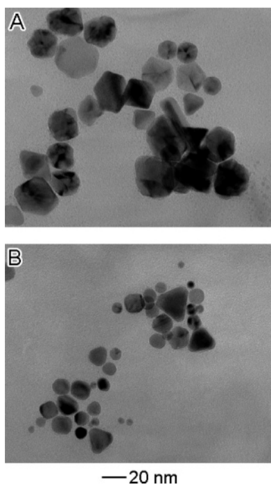
Figure 7. TEM images of two as-synthesized samples illustrating the variation in morphology when different molar ratios between PVP and Pd precursor were used: (A) 1; (B) 25. All other experimental conditions were the same as those used for the synthesis in Figure 1 (at 85 °C in the presence of 0.36 mM FeCl 3 and 5 mM HCl).
